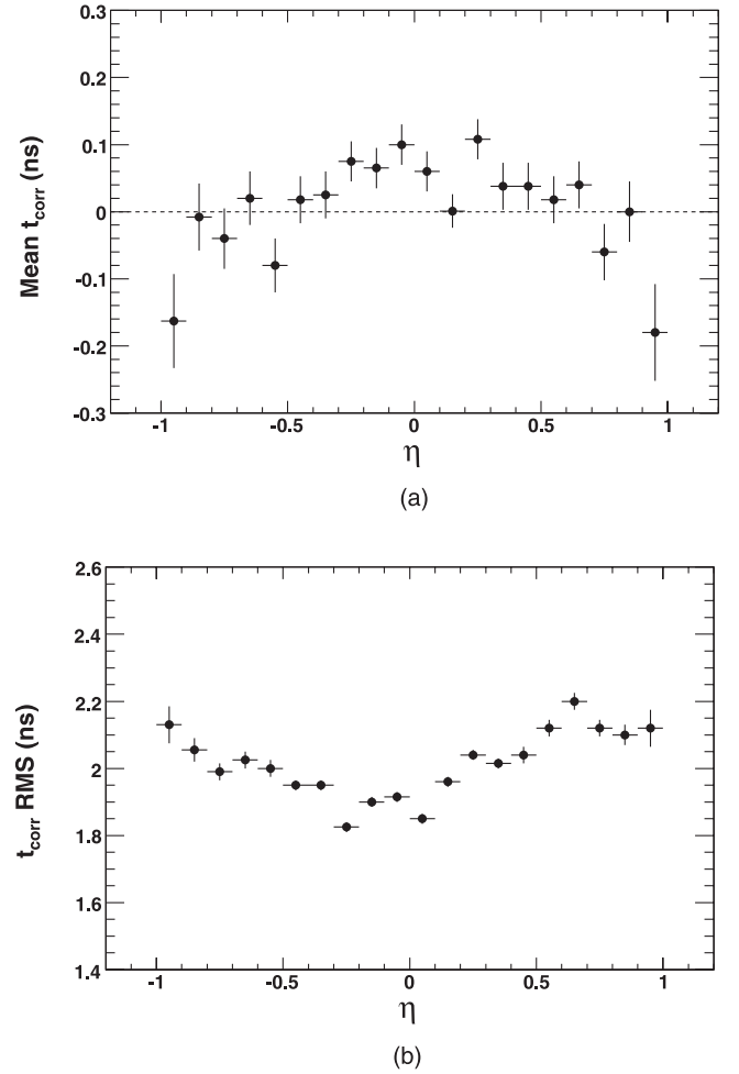
FIG. 15. The mean and RMS of the t_{\text{corr}} distribution for electrons from W \rightarrow e\nu events, where the wrong vertex is picked, as a function of \eta .
