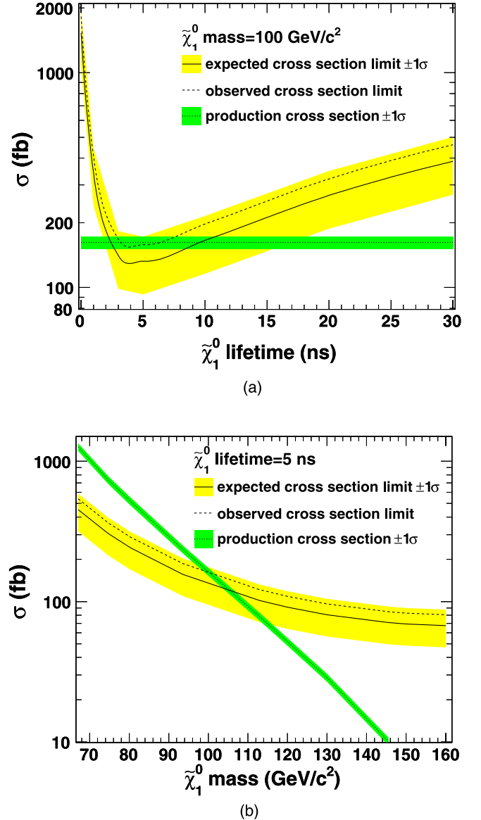
FIG. 23 (color online). The expected and observed cross section limits as a function of the \tilde{\chi}_1^0 lifetime at a mass of 100 \text{GeV}/c^2 (a) and as a function of the \tilde{\chi}_1^0 mass at a lifetime of 5 ns (b). Shaded green (darker shading) is the 6.4% uncertainty-band for the production cross section. The yellow shaded region (lighter shading) is the variation in the expected limit due to the statistical variation on the number of background events in the signal region ( \sim 30\% ).
