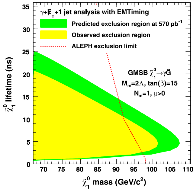
FIG. 25 (color online). The expected and observed 95% C.L. exclusion region along with the most stringent published LEP limits from ALEPH [10]. The highest mass reach of 108 GeV/$c^2$ (expected) and 101 GeV/$c^2$ (observed) is achieved at a lifetime of 5 ns.
