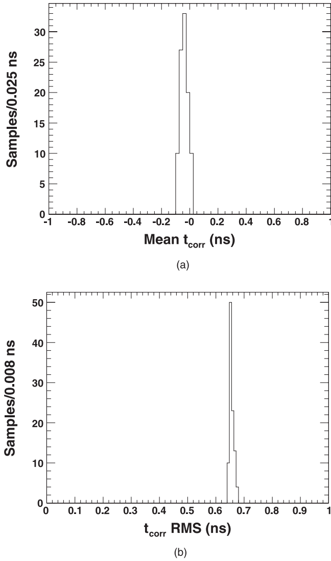
FIG. 14. The mean and RMS of the t_{\text{corr}} distribution for electrons from various subsamples of W \rightarrow e\nu + \text{jets} events where each entry reflects a different combination of the electron E_T , jet E_T , and \cancel{E}_T event requirements. There are slight shifts as the requirements vary. While the mean of the distribution is close to zero, the systematic variation on the mean of the primary Gaussian of the prompt time distribution is conservatively taken to be 0.2 ns in the background estimates.
