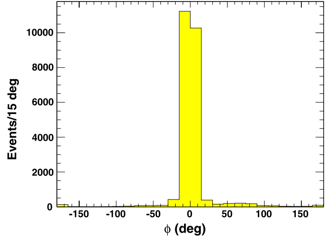
FIG. 19 (color online). The number of beam halo photon candidates as a function of \phi . Most photons arrive at \phi \approx 0 .
