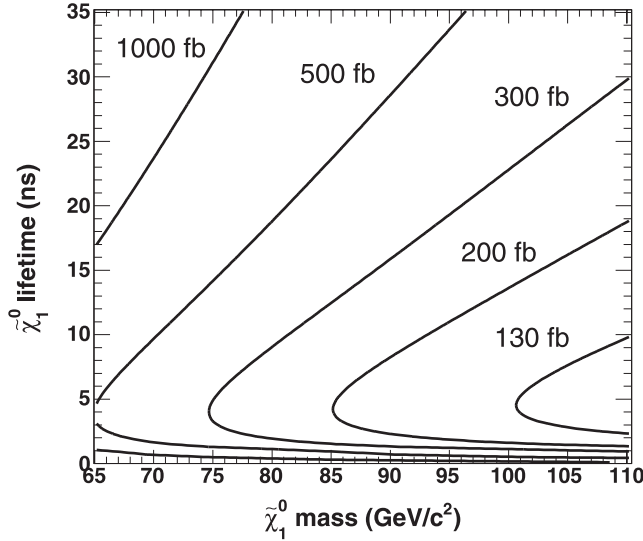
FIG. 24. The contours of constant 95% C.L. cross section upper limit for the observed number of events in the detector.
