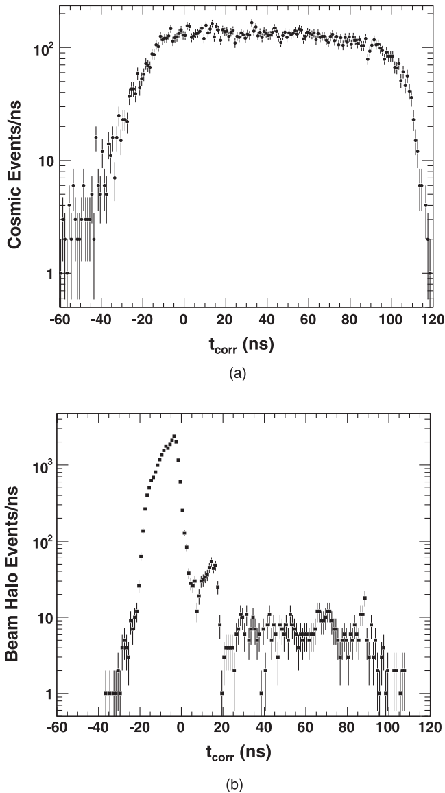
FIG. 18. The t_{\text{corr}} distributions for the cosmic ray (a) and beam halo (b) backgrounds in the \gamma + \cancel{E}_T sample without a collision.
