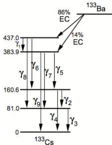
Gamma Emissions
