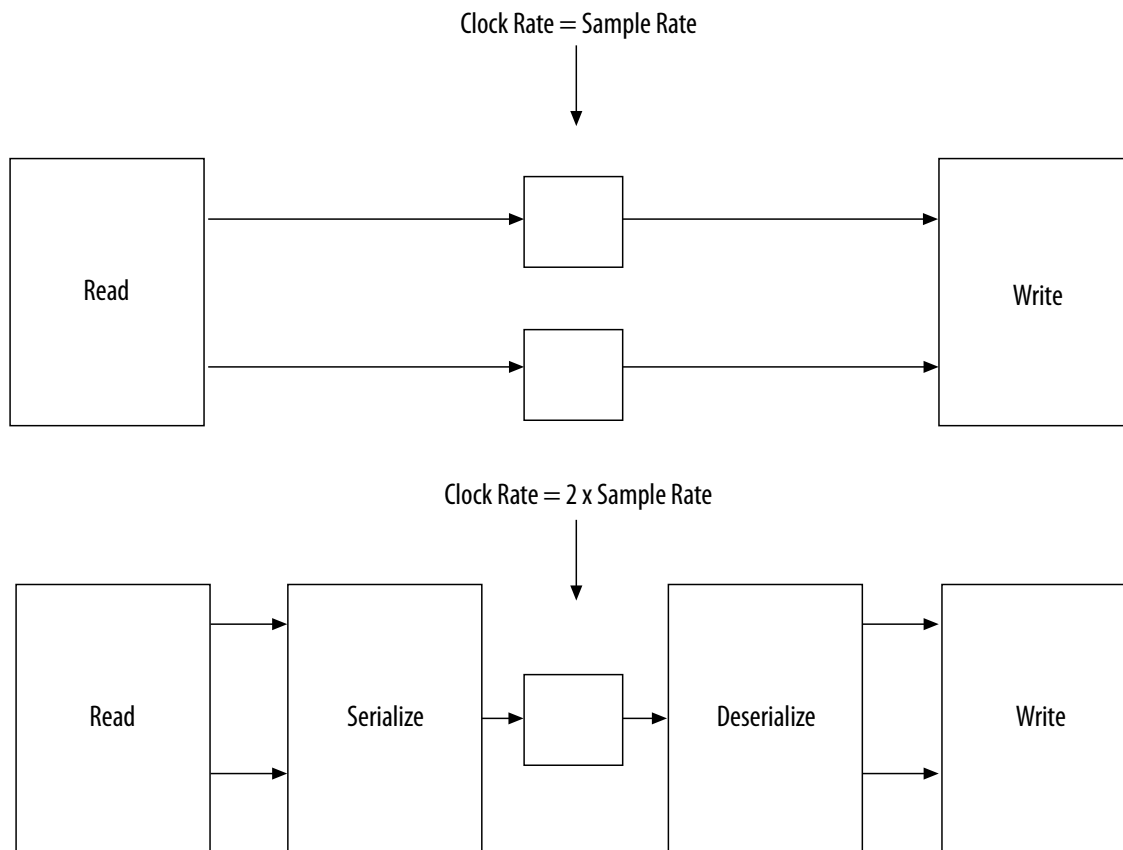
Figure 4-8: Time-Division Multiplexing to Save Hardware Resources
