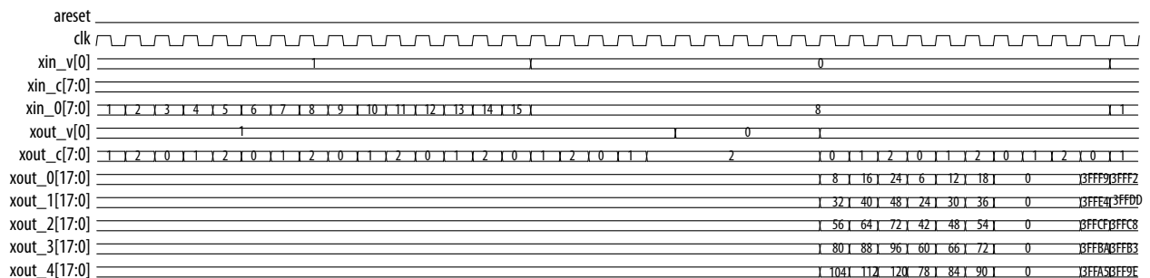
Figure 4-22: Correct Input Format (15 valid cycles, 20 invalid cycles)
