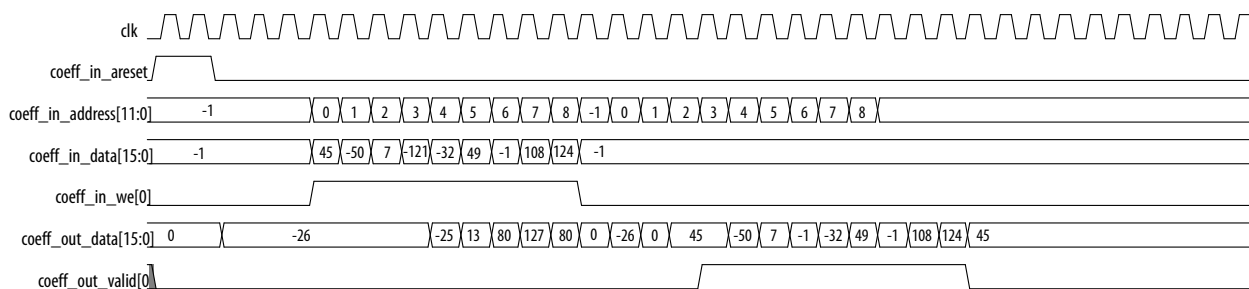
Figure 4-30: Timing Diagram of Coefficient Reloading in Read/Write mode With nine coefficients.
