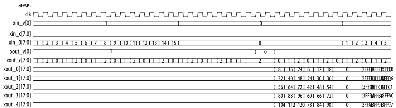
Figure 4-21: Incorrect Input Format (15 valid cycles, 0 invalid cycles) If the number of invalid cycles is less than 17, the output format is incorrect,
