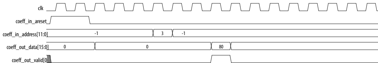
Figure 4-33: Timing Diagram of Multiple Coefficient Banks
