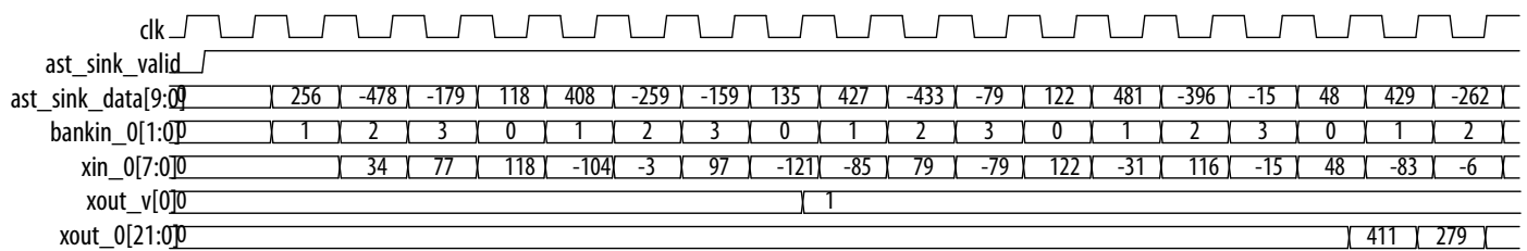
Figure 4-29: Timing Diagram of a Four-Channel Filter with 4 Coefficient Banks Each channel has a separate corresponding coefficient set. The bank inputs for different channels are driven with their channel number respectively throughout the filter operation
