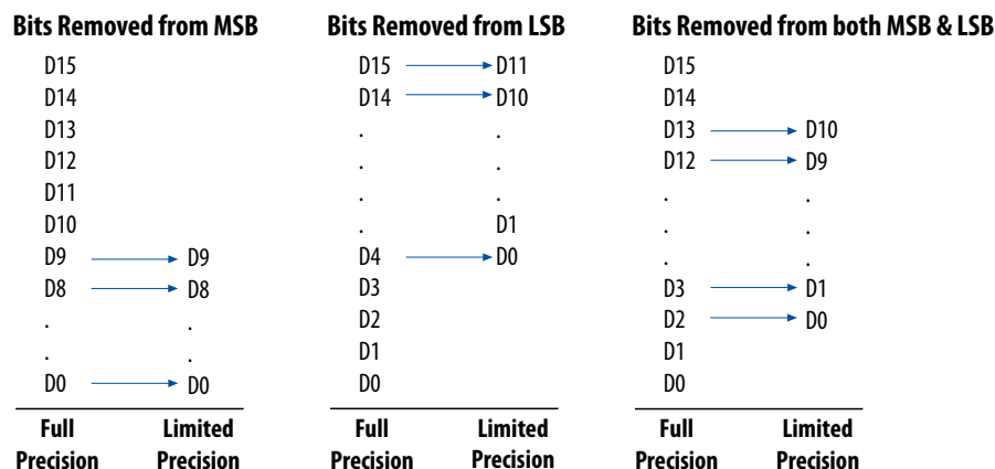
Figure 3-1: Removing Bits from the MSB and LSB
