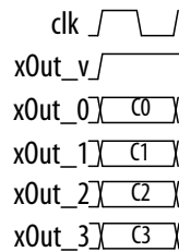
Figure 4-17: Four Channels on Four Wires (Output)
