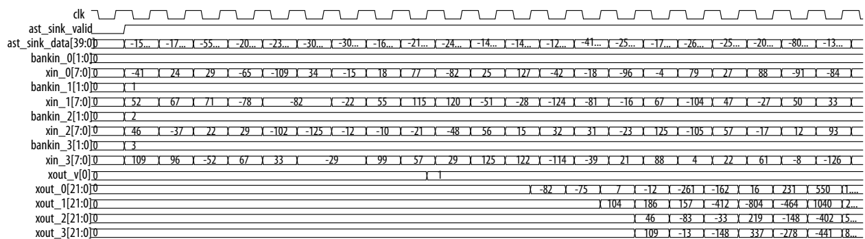
Figure 4-29: Timing Diagram of a Four-Channel Filter with 4 Coefficient Banks Each channel has a separate corresponding coefficient set. The bank inputs for different channels are driven with their channel number respectively throughout the filter operation
