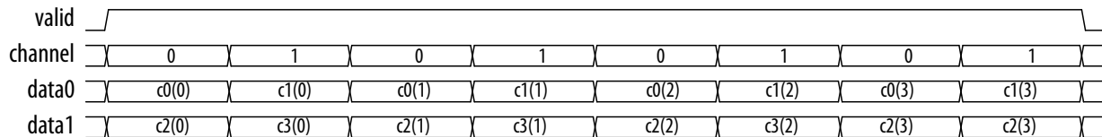
Figure 4-12: Four Channels on Two Wires with No Invalid Cycles
