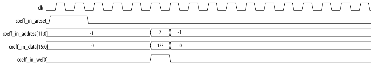
Figure 4-32: Timing Diagram of Coefficient Reloading in Read mode
