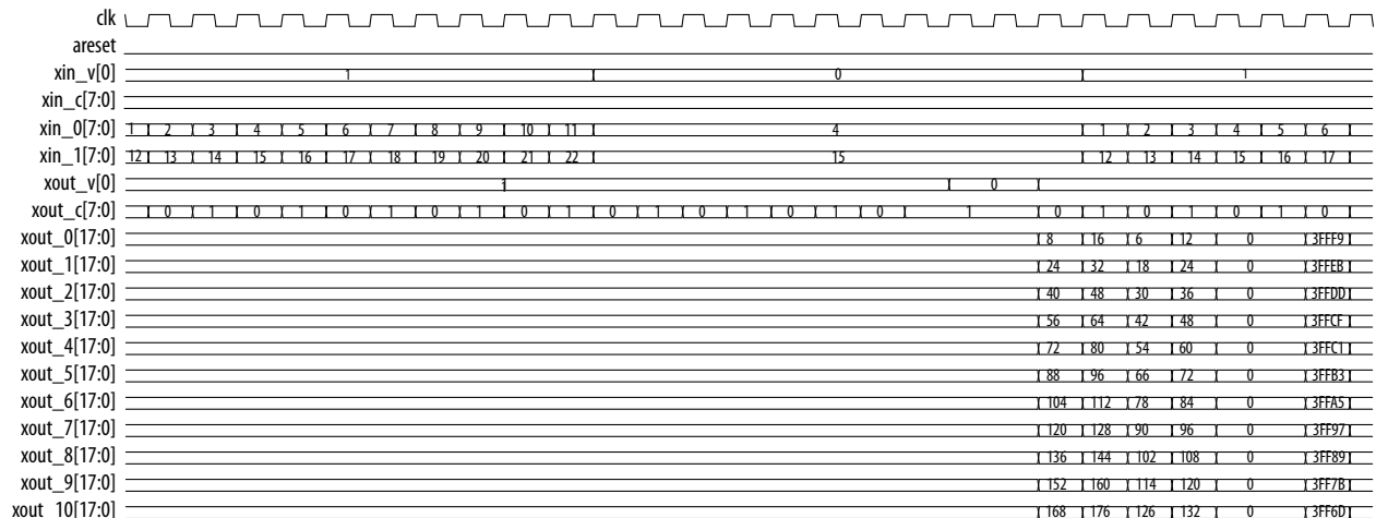
Figure 4-25: Correct Input Format (11 valid cycles, 11 invalid cycles)
