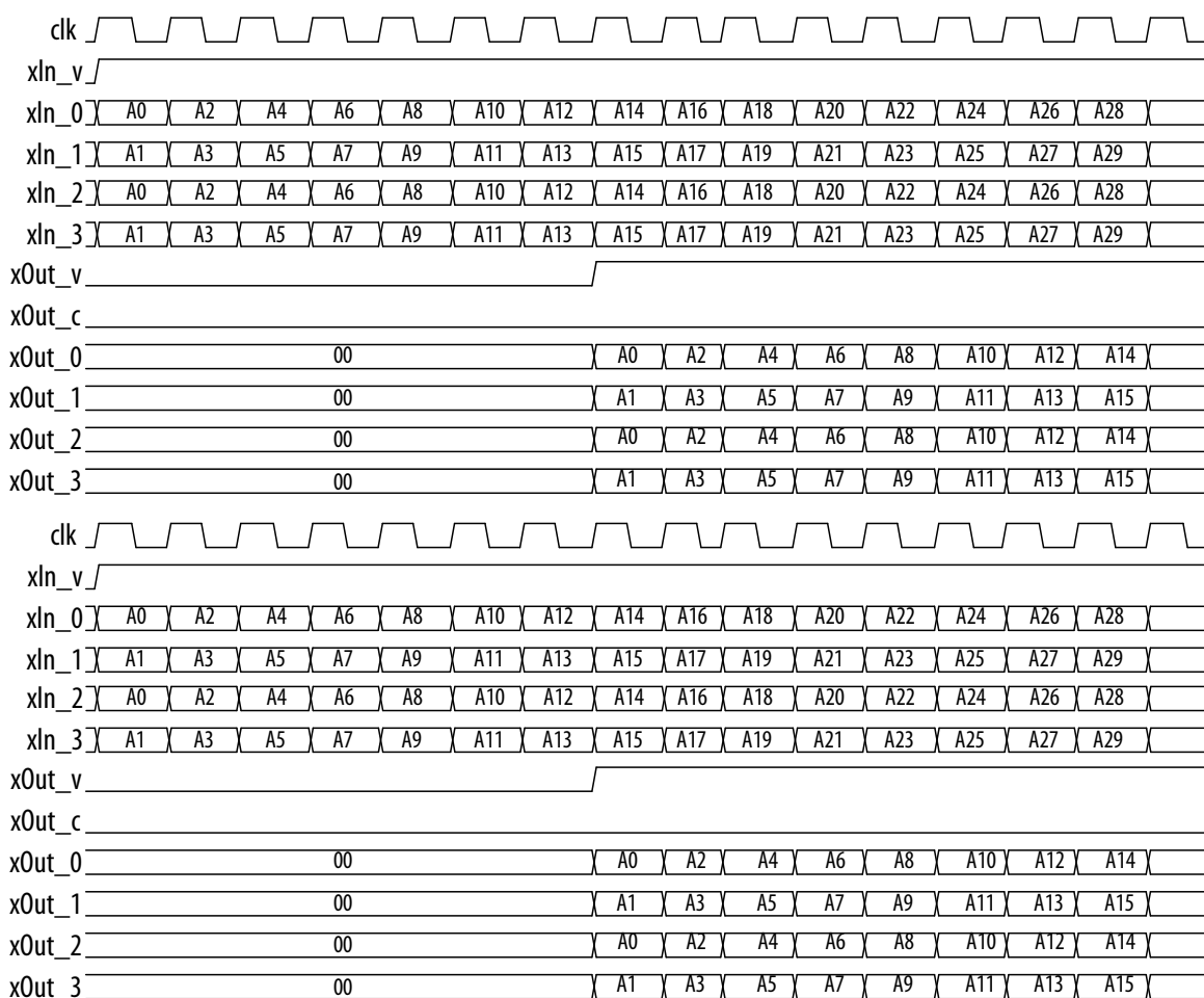
Figure 4-27: Super Sample Rate Filter (clkRate=100, inputRate=200) with inChans=2If inputChannelNum = 2
