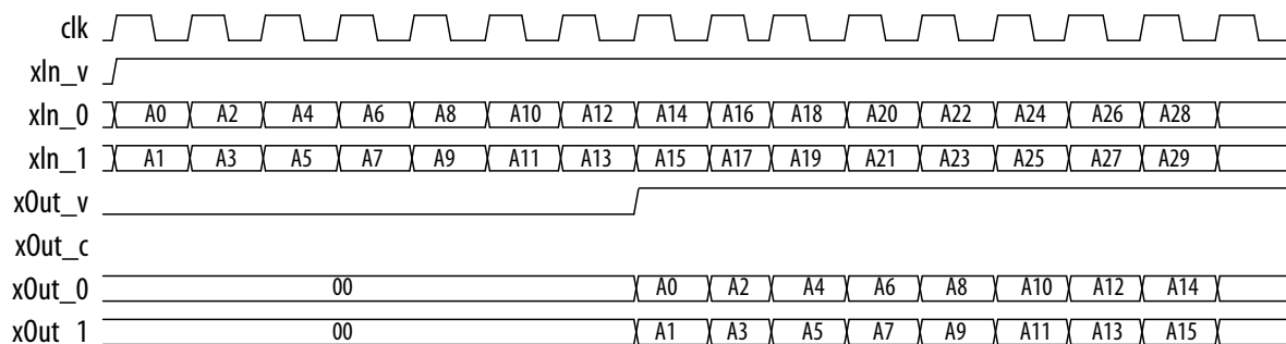
Figure 4-26: Super Sample Rate Filter (clkRate=100, inputRate=200) with inChans=1A0 is the first sample of channel A, A1 is the second sample of channel A, and so forth.
