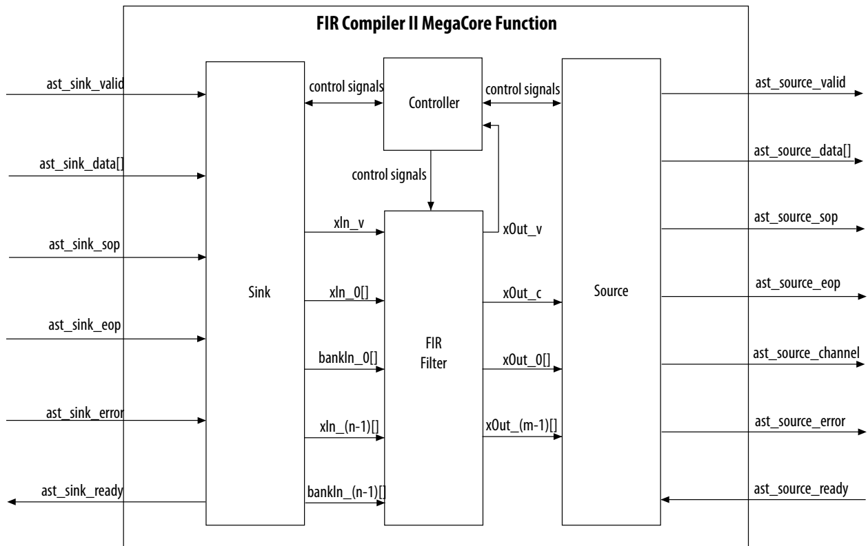
Figure 4-1: High Level Block Diagram of FIR II IP core with Avalon-ST Interface
