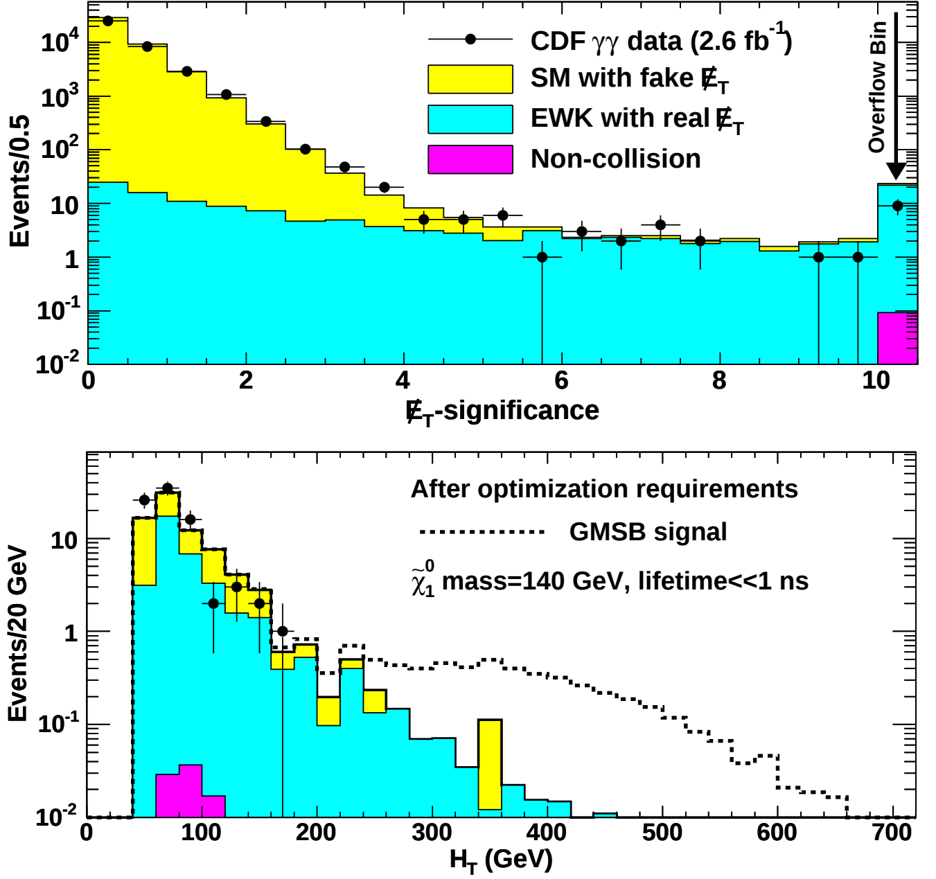
FIG. 1: The top plot shows the E_T -significance distribution for the inclusive \gamma\gamma candidate sample, along with the background predictions. The bottom plot shows the predicted H_T distribution after all but the final H_T requirement.
