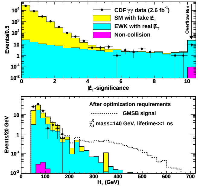
FIG. 1: The top plot shows the \cancel{E}_T -significance distribution for the inclusive \gamma\gamma candidate sample, along with the background predictions. The bottom plot shows the predicted H_T distribution after all but the final H_T requirement.
