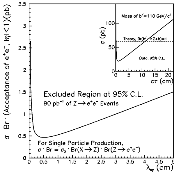
FIG. 3. The 95% confidence level upper cross section limit for \sigma \cdot B times the acceptance for an electron-positron pair to be within the detector as a function of fixed \lambda_{xy} . Cross sections above the curve have been excluded at the 95% confidence level. The inset shows the exclusion curve and the theoretical prediction for a b' quark of mass 110 \text{ GeV}/c^2 as a function of its lifetime, assuming 100% decay into Z^0 b .
