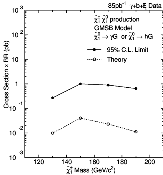
FIG. 11. The limits on the cross section times branching ratio for the SUSY production of \gamma b \tilde{E}_t events in the GMSB model. All production processes have been included.
