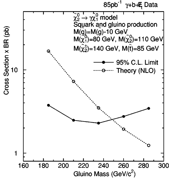
FIG. 9. The limits on the cross section times the branching ratio for SUSY production of \gamma b \cancel{E}_t events in the \tilde{\chi}_2^0 \rightarrow \gamma \tilde{\chi}_1^0 model. All production processes have been included; the dominant mode is the production of squarks and gluinos which decay to charginos and neutralinos. The overall branching ratio to the \gamma b \cancel{E}_t topology is approximately 30%.
